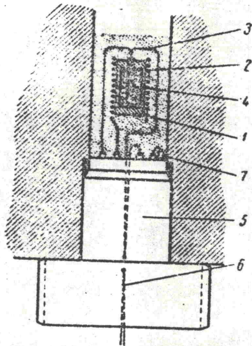
Fig. 1. Schematic cross-section of the measuring device inside the canal of a super high-pressure vessel.
