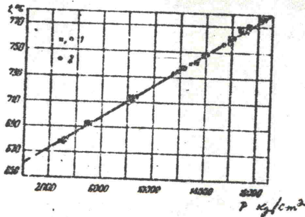
Fig. 2. Pressure dependence of the melting point of aluminum:
